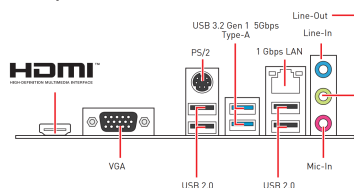
Rear I/O Panel
